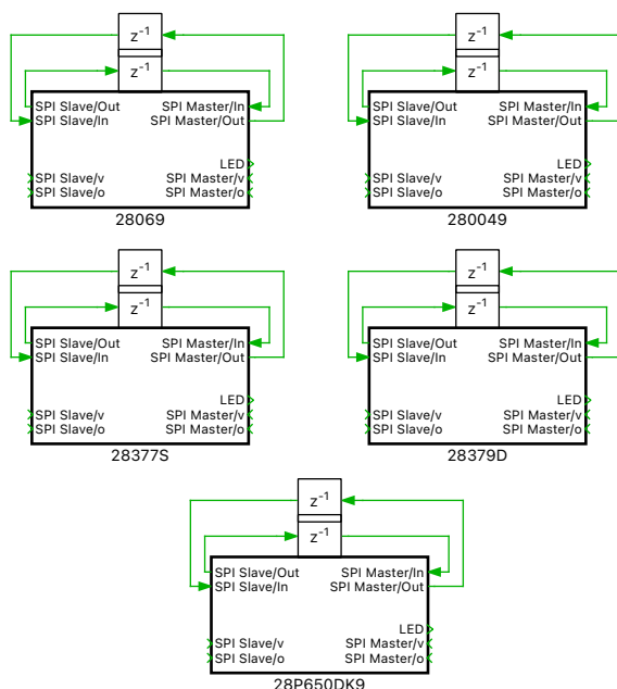
Figure 1: Top level schematic of the model with four subsystems
