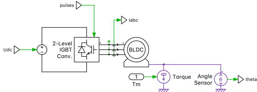
Figure 1: Brushless DC machine circuit
