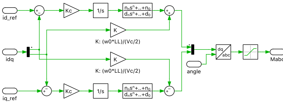
Figure 3: Current controller
